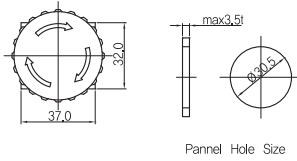
Pannel Hole Size
