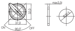
Panel Hole Size
